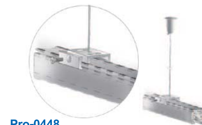
Pro-0448 懸掛裝置 (帶1.5m鋼線)
